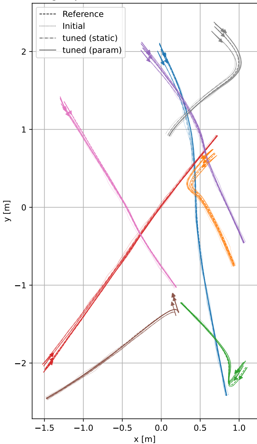
Training Trajectories (8 shown, 4 start offsets each)
